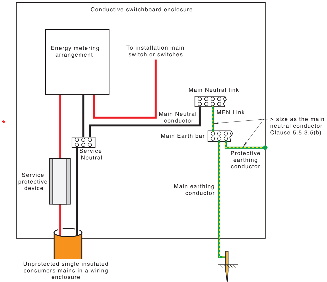
FIGURE 5.6(B) EARTHING ARRANGEMENT FOR CONDUCTIVE SWITCHBOARD ENCLOSURES ASSOCIATED WITH UNPROTECTED CONSUMER MAINS [CLAUSE 5.5.3.5(b)]
