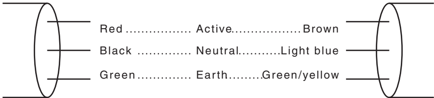
FIGURE 3.1 SINGLE-PHASE CABLES
