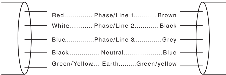
FIGURE 3.2 MULTIPHASE CABLES
