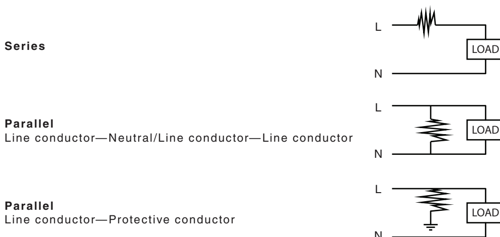
FIGURE O1 TYPES OF ARC FAULT
