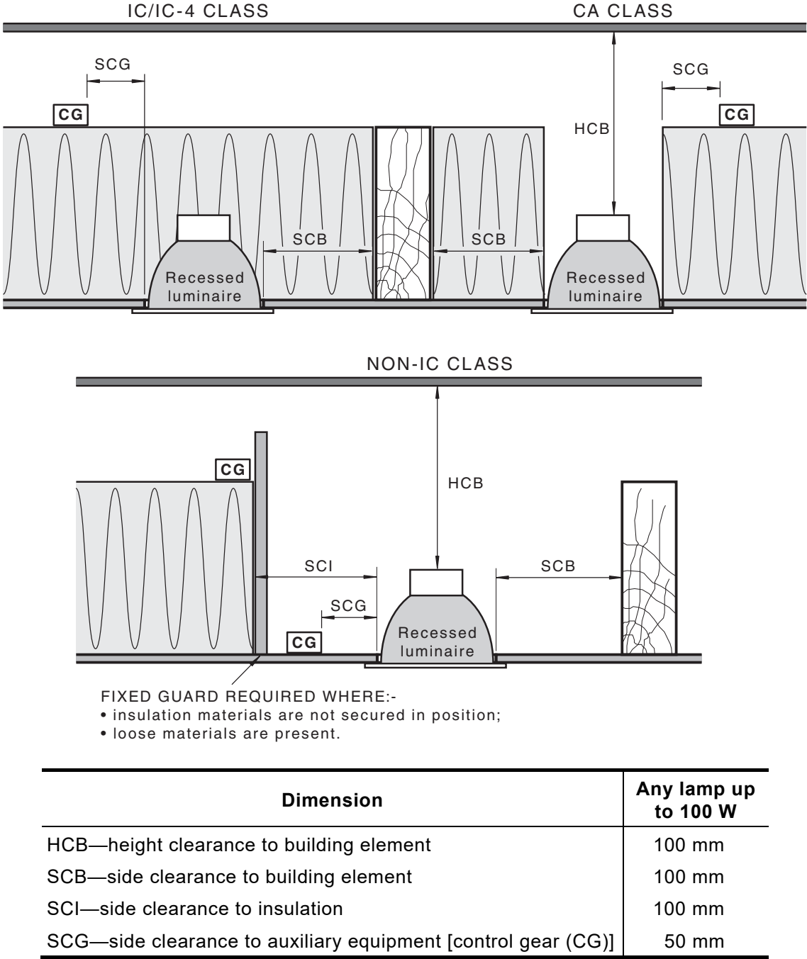
FIGURE 4.9 DEFAULT MINIMUM CLEARANCES FOR RECESSED LUMINAIRES
