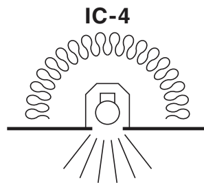
FIGURE 4.16 IC-4 SYMBOL
